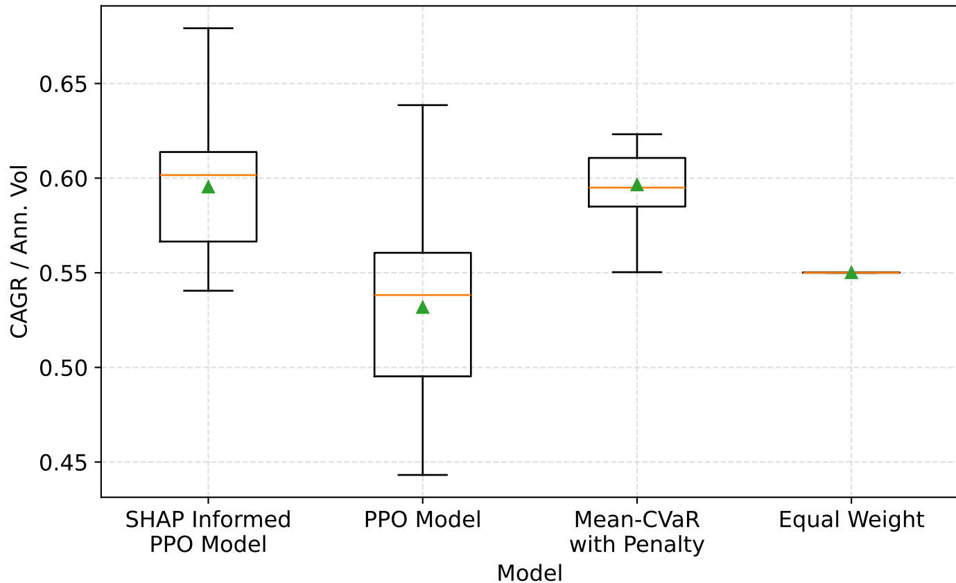
Sector ETFs: Return/Vol — Distribution Across 30 Iterations
